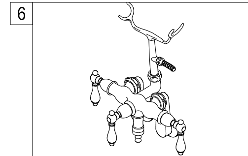
6. Place a washer between the side hole of the shower cradle and the cone nut of the shower hose. Tighten the cone nut.
