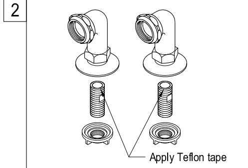
2. Apply Teflon tape on the threads of the copper shank. Install the risers.
