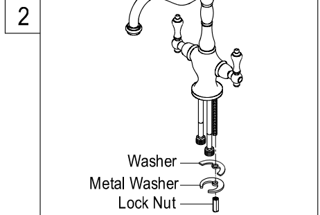
2. Insert the inlet shanks through the sink holes, and press down. Assemble the washers and locknuts on the inlet shanks, and then tighten the nuts by basin wrench.
