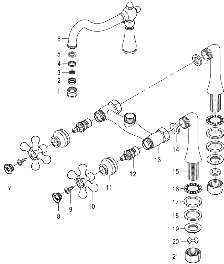
Hot Cartridge: KC1000H
